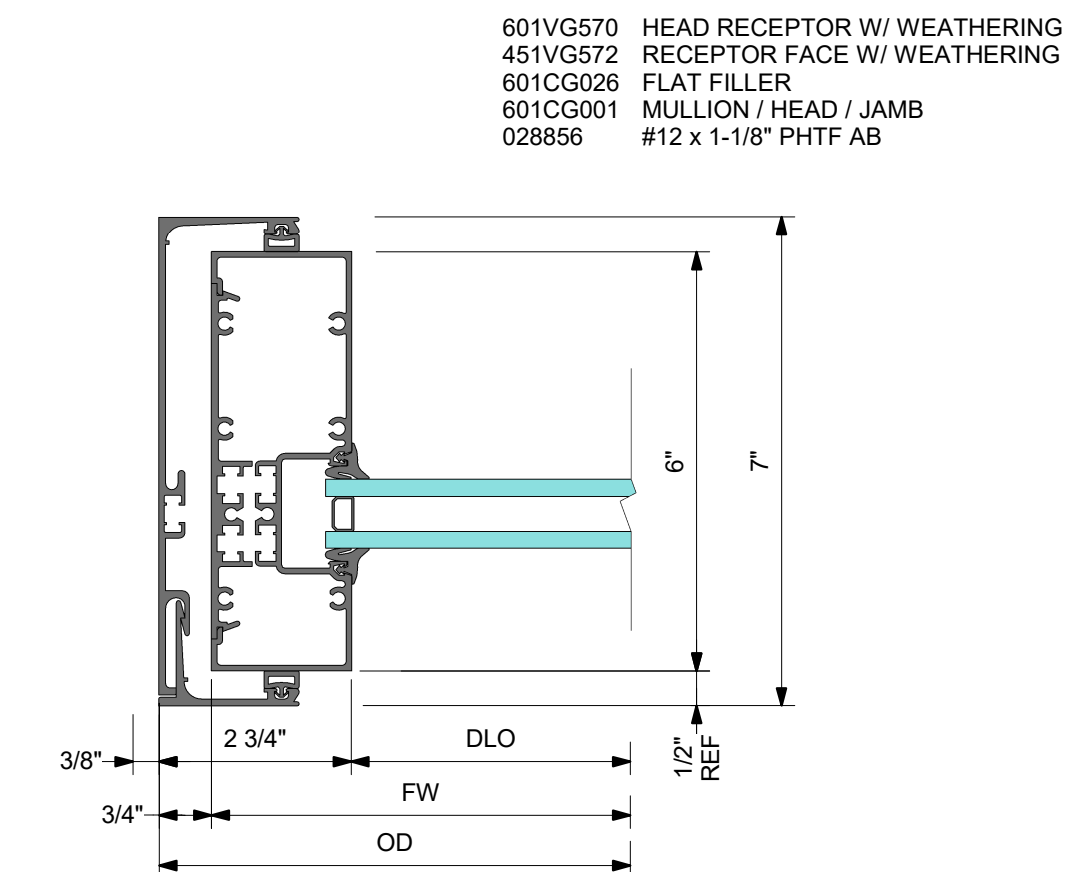
4 DETAIL 4 JAMB WITH RECEPTOR
