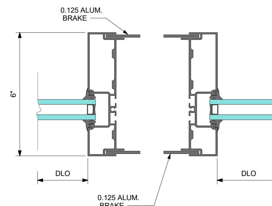
601CG010 FEMALE EXPANSION MULLION HALF
