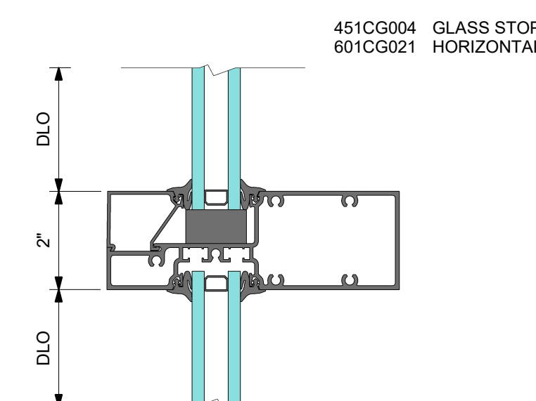
2 DETAIL 2 HORIZONTAL
