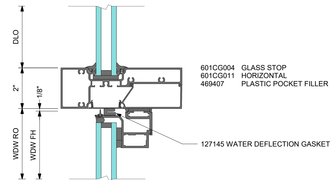
1 VENT HEAD
