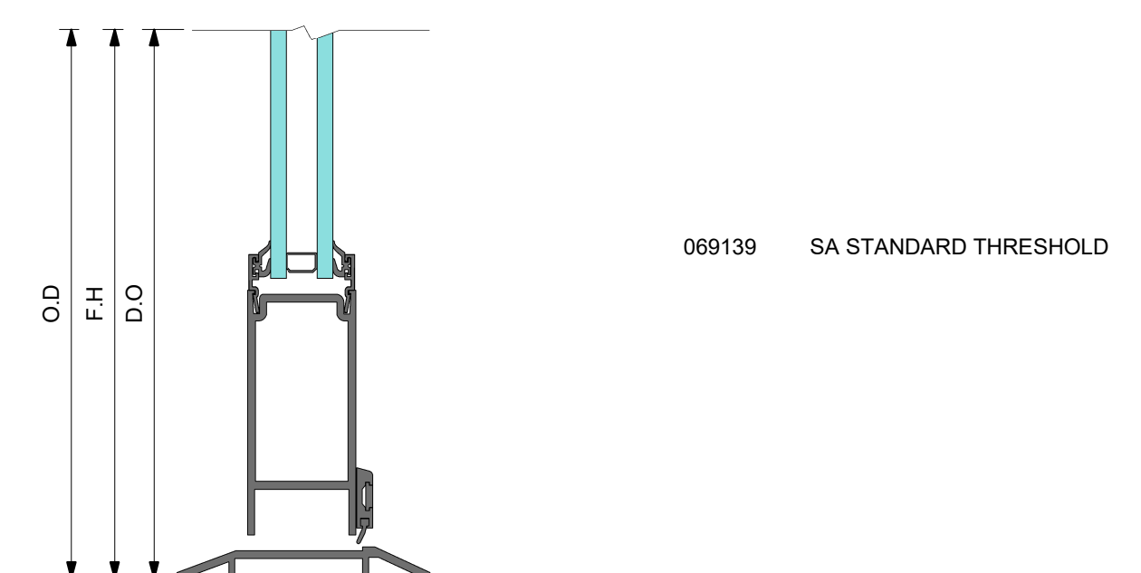
3 DETAIL 3 THRESHOLD
