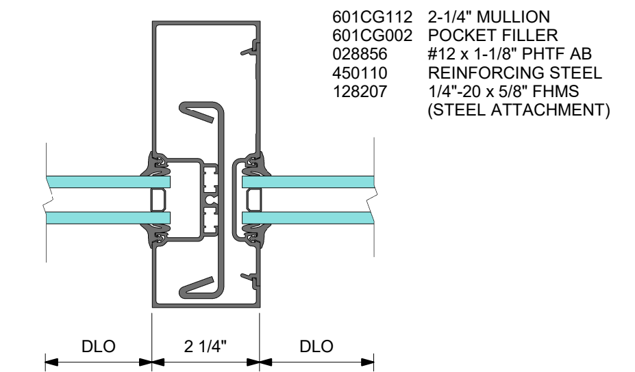
5 DETAIL 5 - 2-1/4" VERTICAL MULLION WITH STEEL
