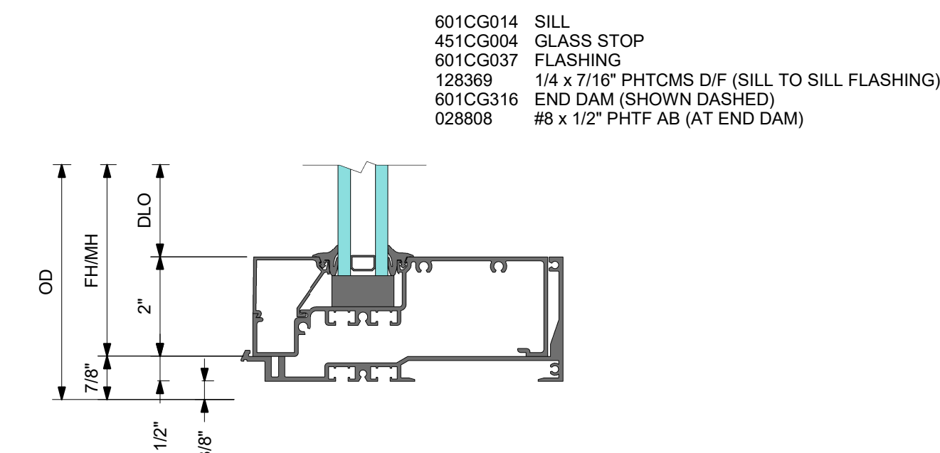
3 DETAIL 3 SILL
