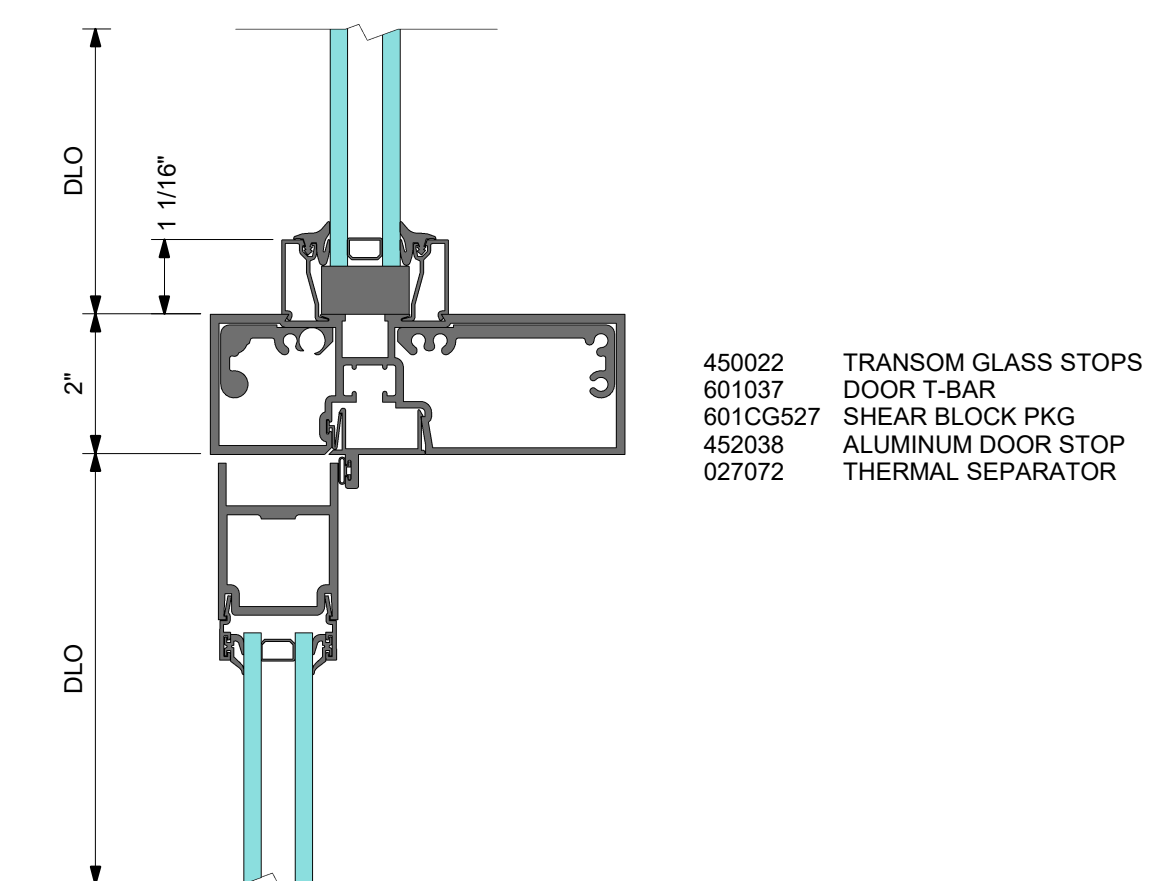
2 DETAIL 2 TRANSOM BAR WITH SURFACE CLOSER
