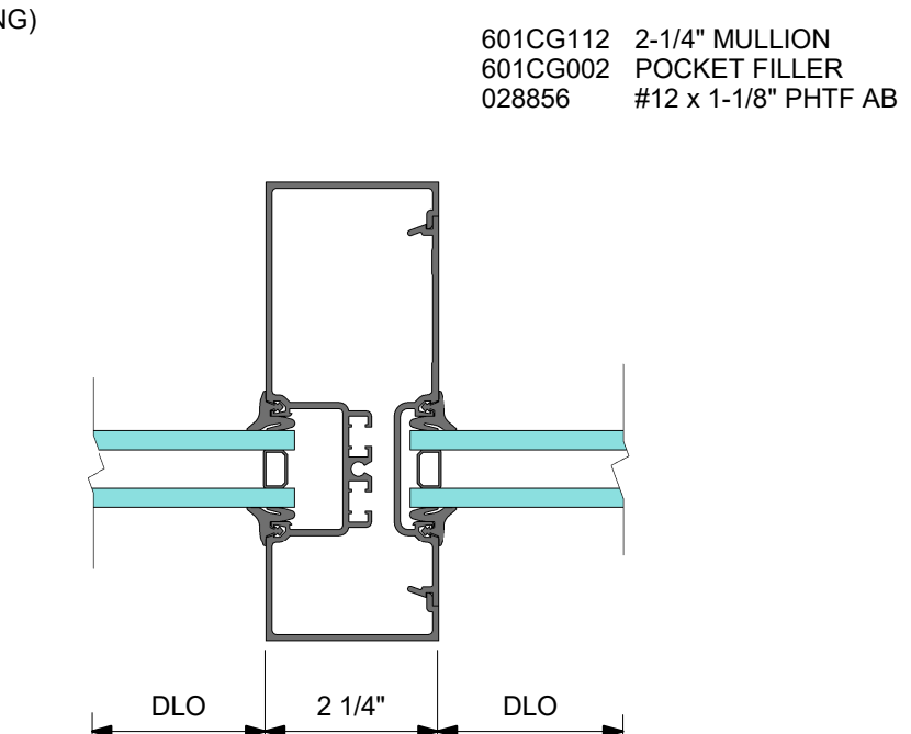
6 DETAIL 6 - 2-1/4" VERTICAL MULLION
