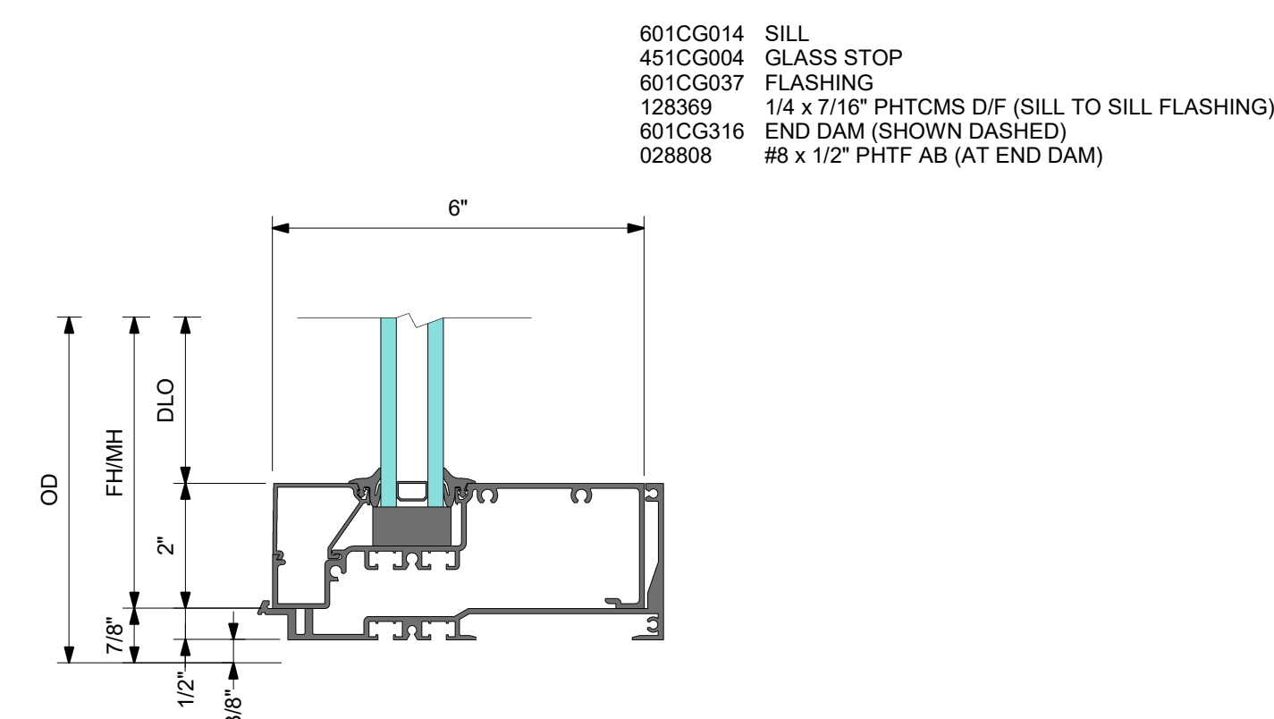
3 DETAIL 3 SILL
