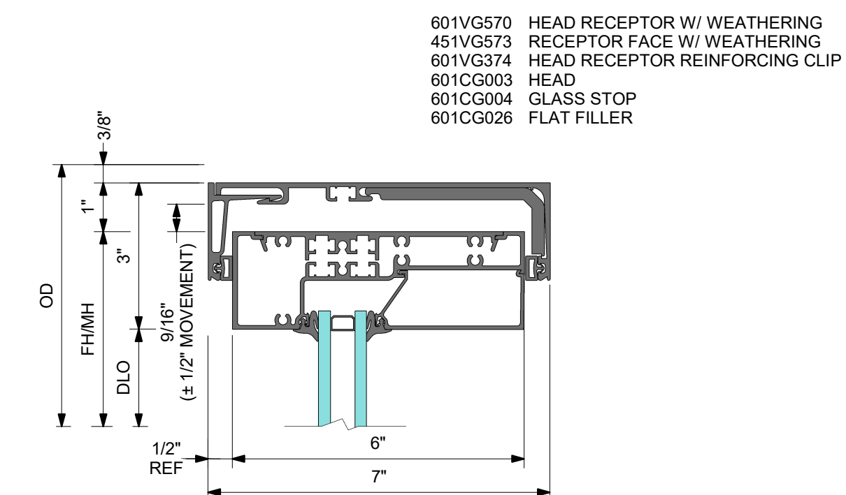
1 DETAIL 1 HEAD WITH HD RECEPTOR
