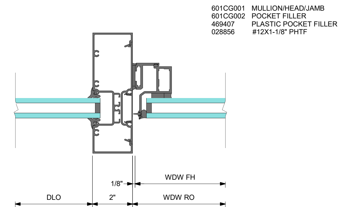
3 VENT @ RIGHT
