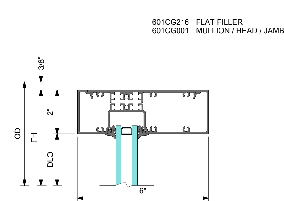
1 DETAIL 1 HEAD
