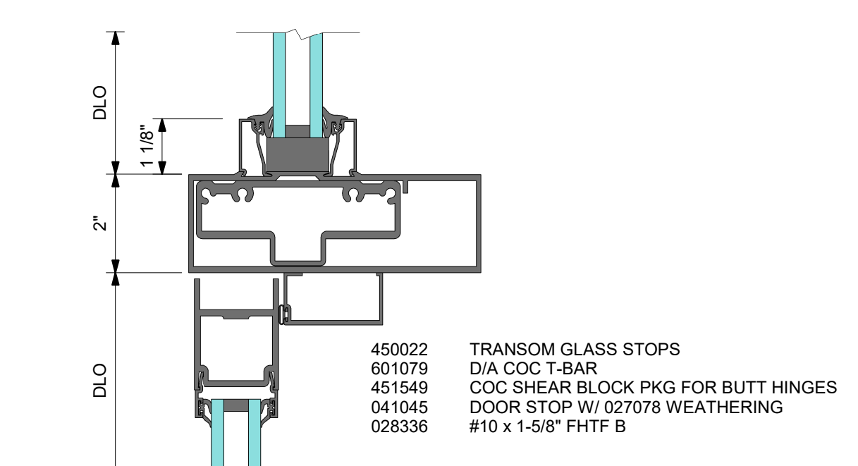
DOOR TRANSOM BAR WITH KAWNEER CONCEALED CLOSER AND OFFSET PIVOTS
