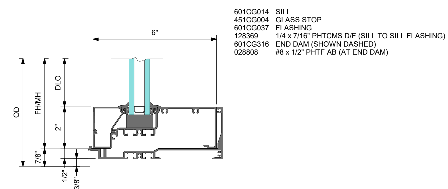
3 DETAIL 3 SILL
