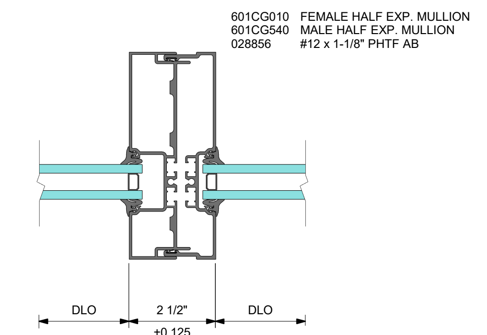
6 DETAIL 6 EXPANSION MULLION
