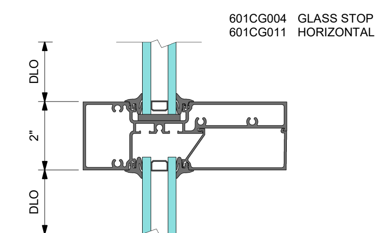
2 DETAIL 2 HORIZONTAL
