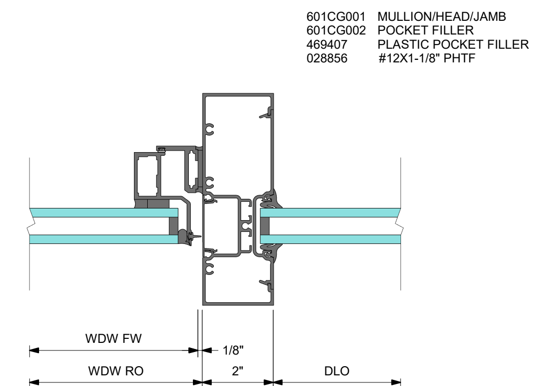
4 VENT @ LEFT
