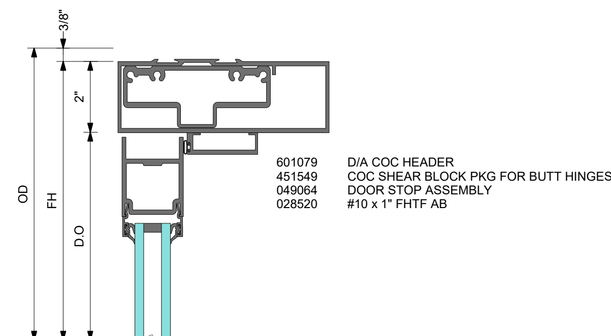
DOOR HEADER WITH LCN CONCEALED CLOSER AND BUTT HINGES
