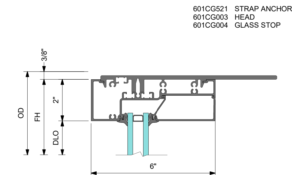
1 DETAIL 1 HEAD WITH STRAP ANCHOR
