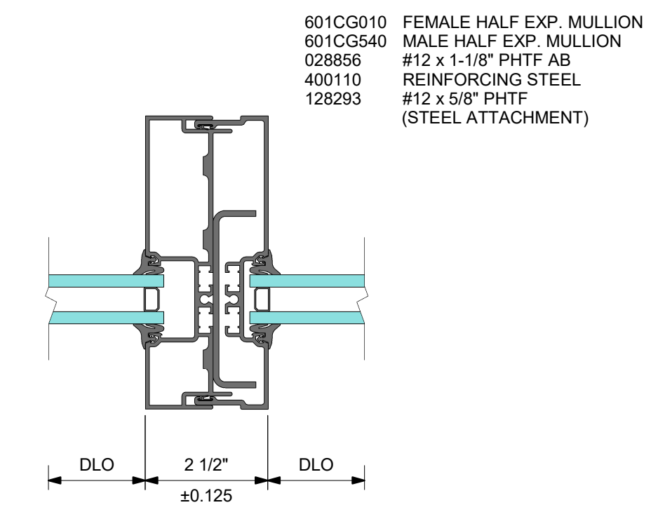
5 DETAIL 5 EXPANSION MULLION WITH STEEL
