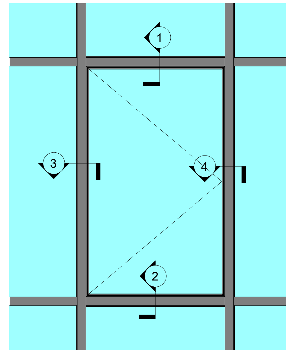
OUTSWING CASEMENT
