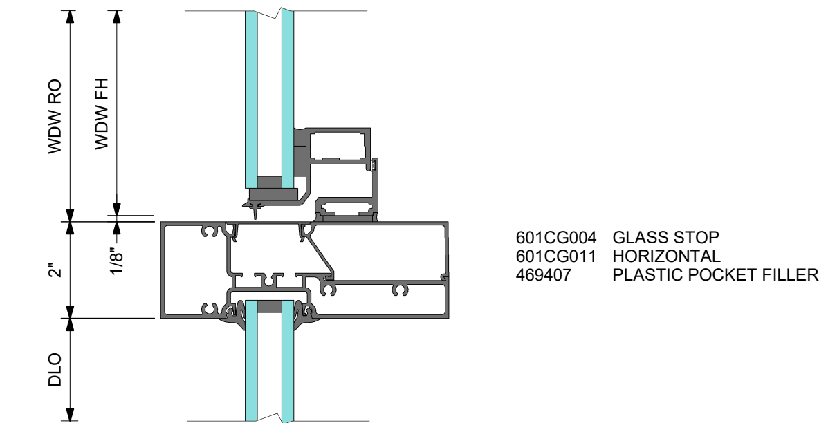
2 VENT SILL
