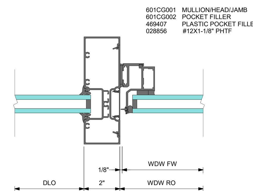
3 VENT @ RIGHT
