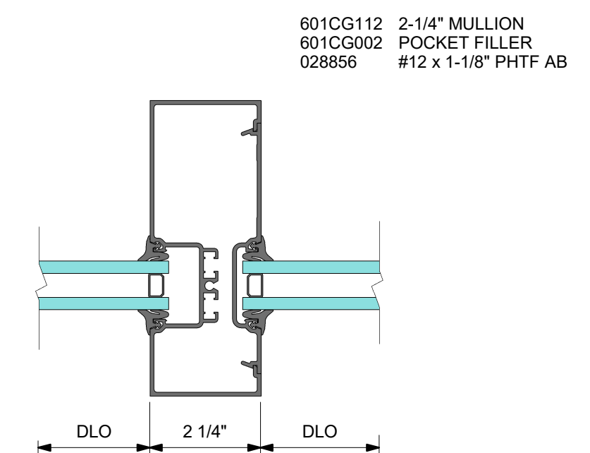
6 DETAIL 6 - 2-1/4" VERTICAL MULLION
