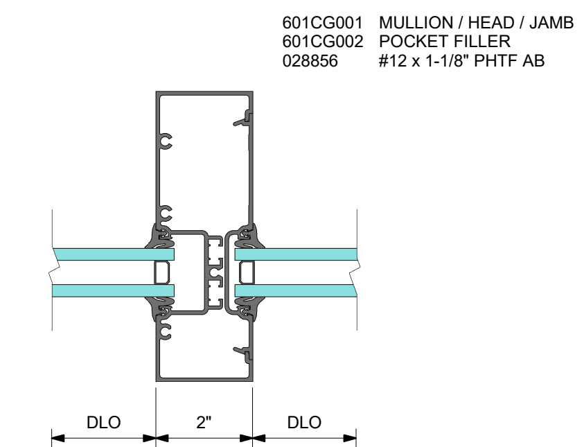
5 DETAIL 5 VERTICAL MULLION
