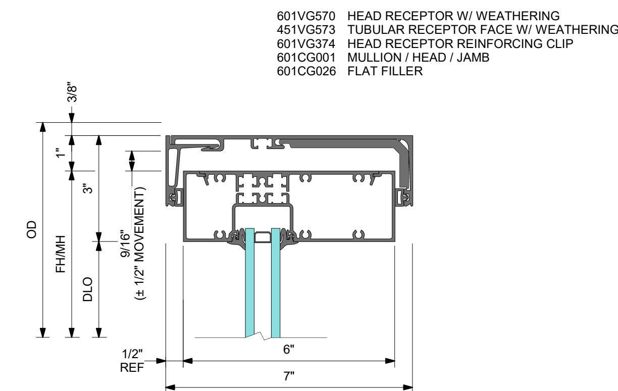
1 DETAIL 1 HEAD WITH HD RECEPTOR
