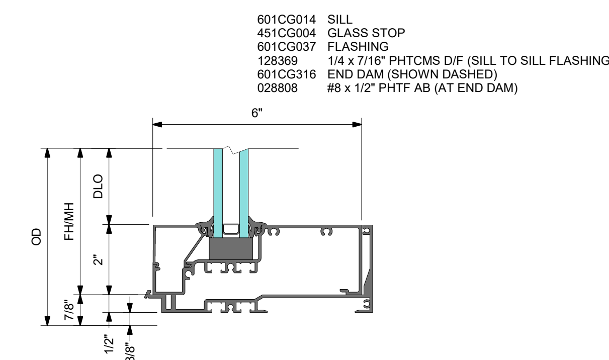
3 DETAIL 3 SILL
