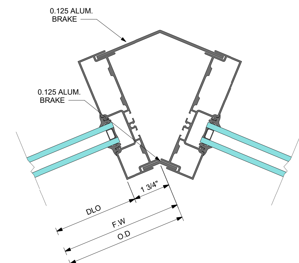
135° INSIDE CORNER WITH BRAKE METAL
