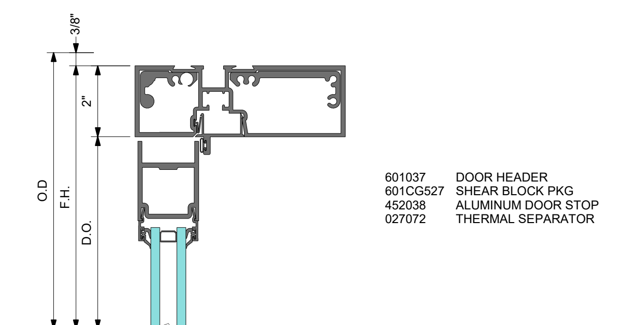
2A DETAIL 2A TRANSOM BAR WITH SURFACE CLOSER
