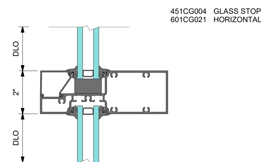
2 DETAIL 2 HORIZONTAL
