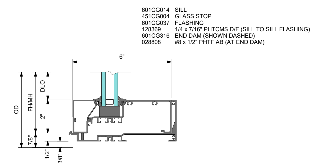
3 DETAIL 3 SILL
