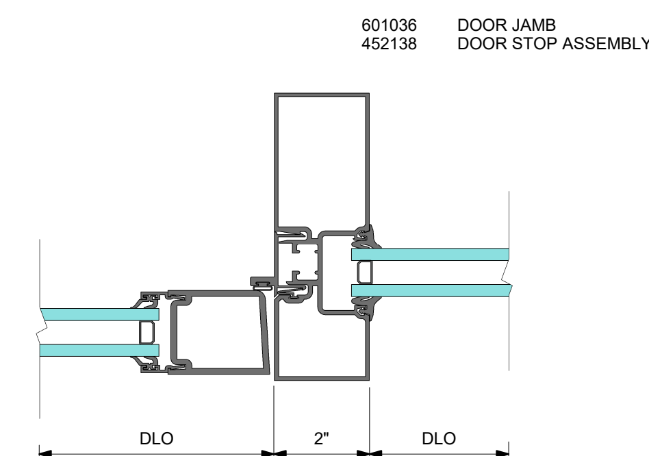
5 DETAIL 5 DOOR JAMB WITH SIDELITE
