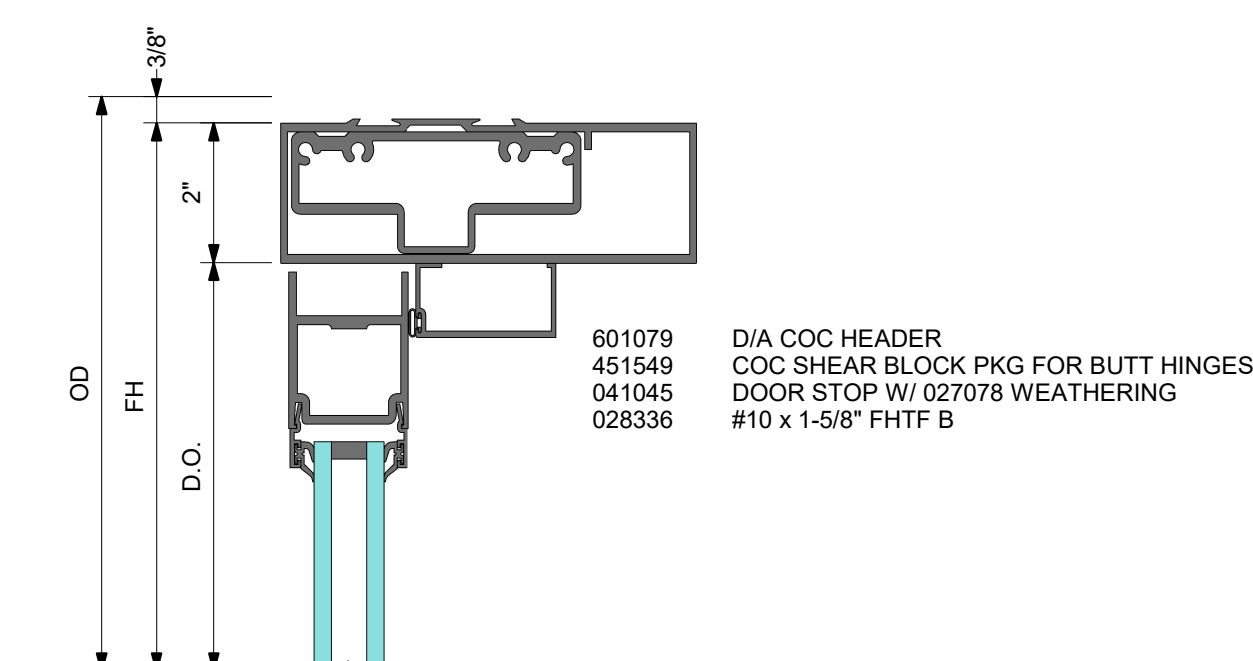
DOOR HEADER WITH KAWNEER CONCEALED CLOSER AND BUTT HINGES
