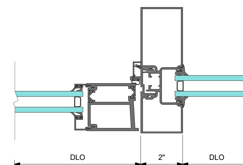
5 DETAIL 5 DOOR JAMB WITH SIDELITE
