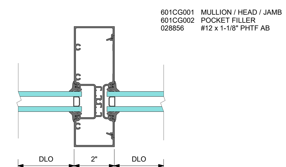
5 DETAIL 5 VERTICAL MULLION
