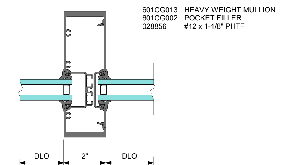
5 DETAIL 5 HEAVY WEIGHT VERTICAL MULLION
