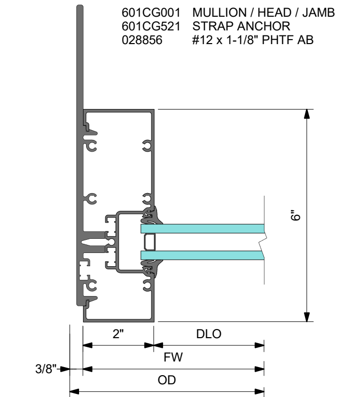
4 DETAIL 4 JAMB WITH STRAP ANCHOR
