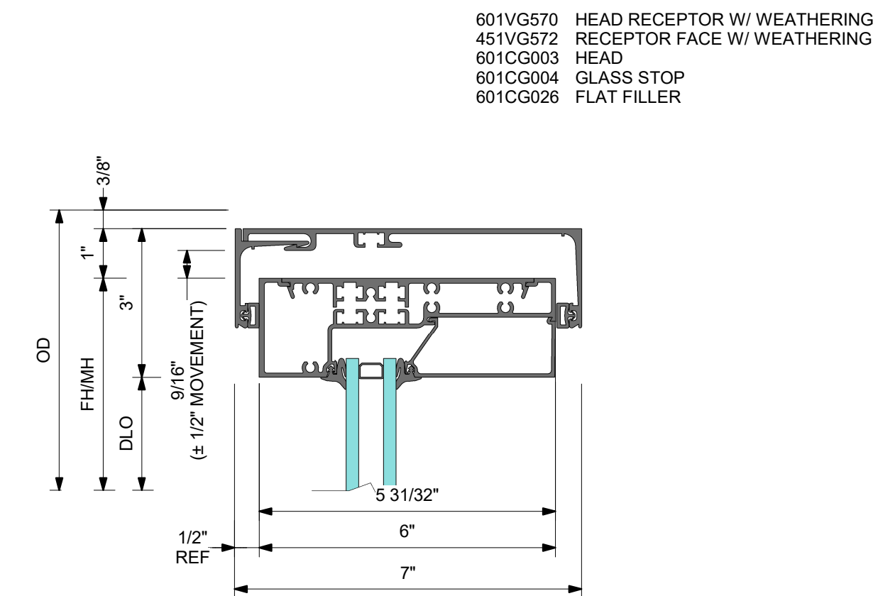
1 DETAIL 1 HEAD WITH RECEPTOR
