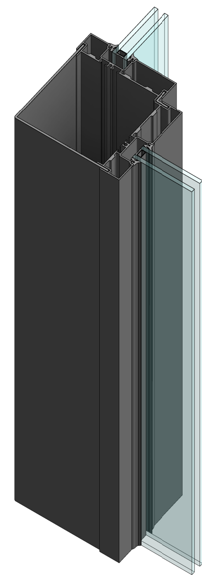
3D-VIEW
