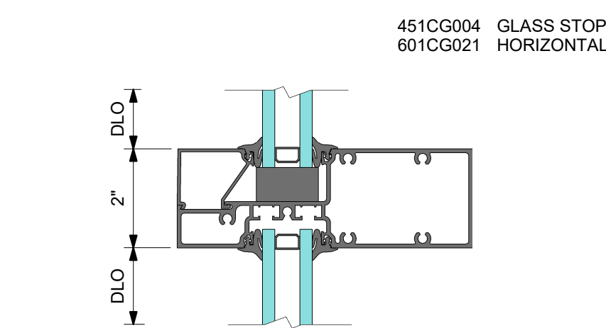
2 DETAIL 2 HORIZONTAL
