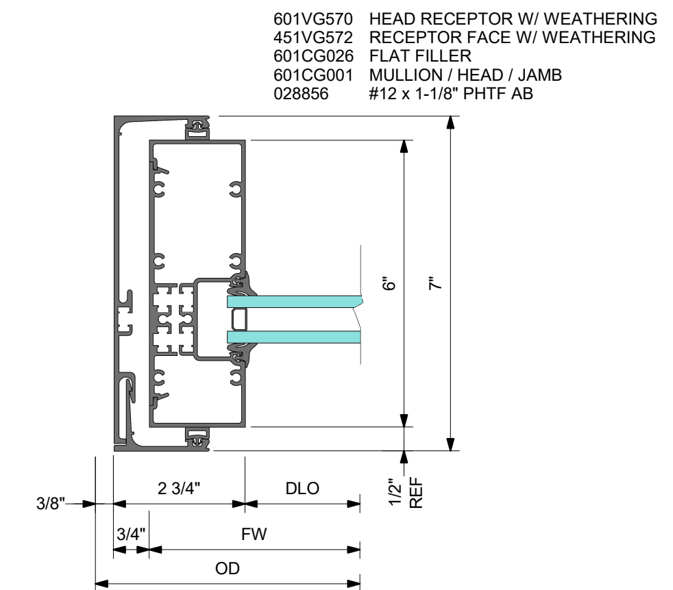
4 DETAIL 4 JAMB WITH RECEPTOR
