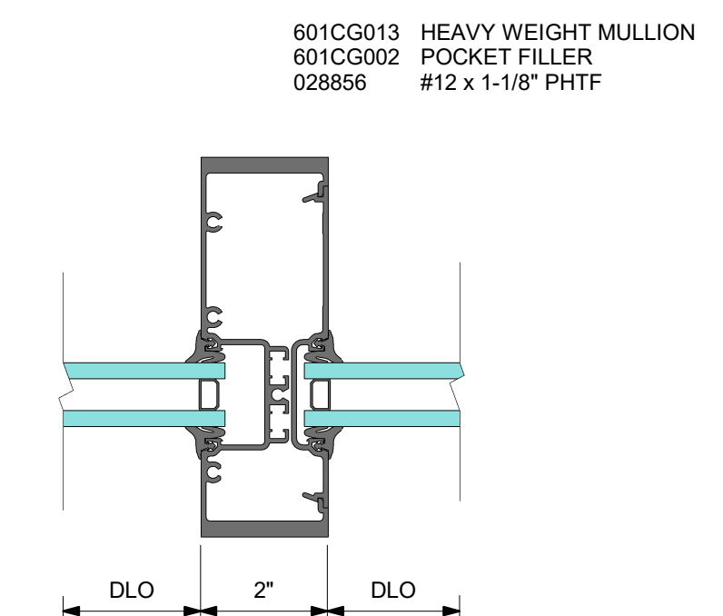
5 DETAIL 5 HEAVY WEIGHT VERTICAL MULLION
