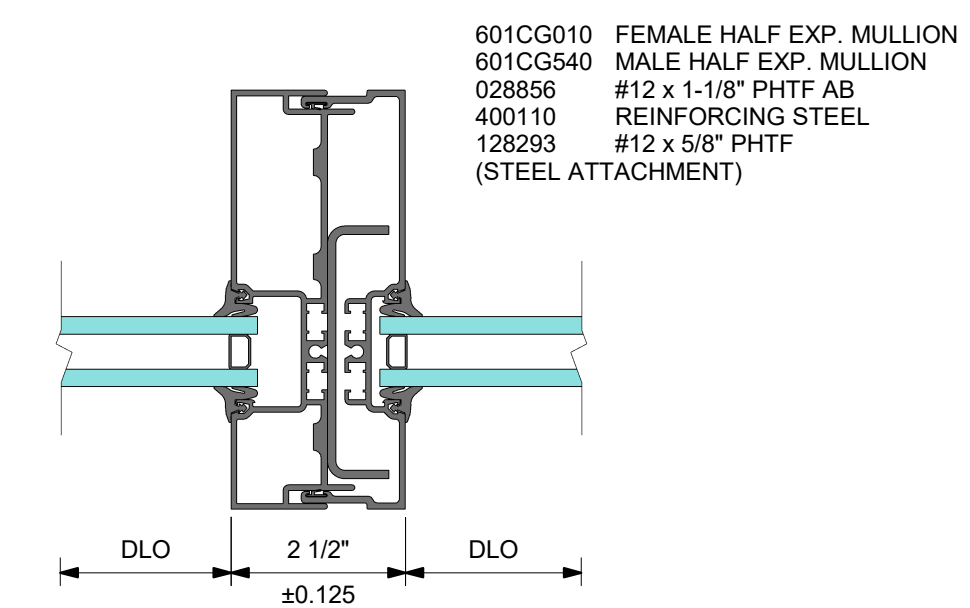
5 DETAIL 5 EXPANSION MULLION WITH STEEL
