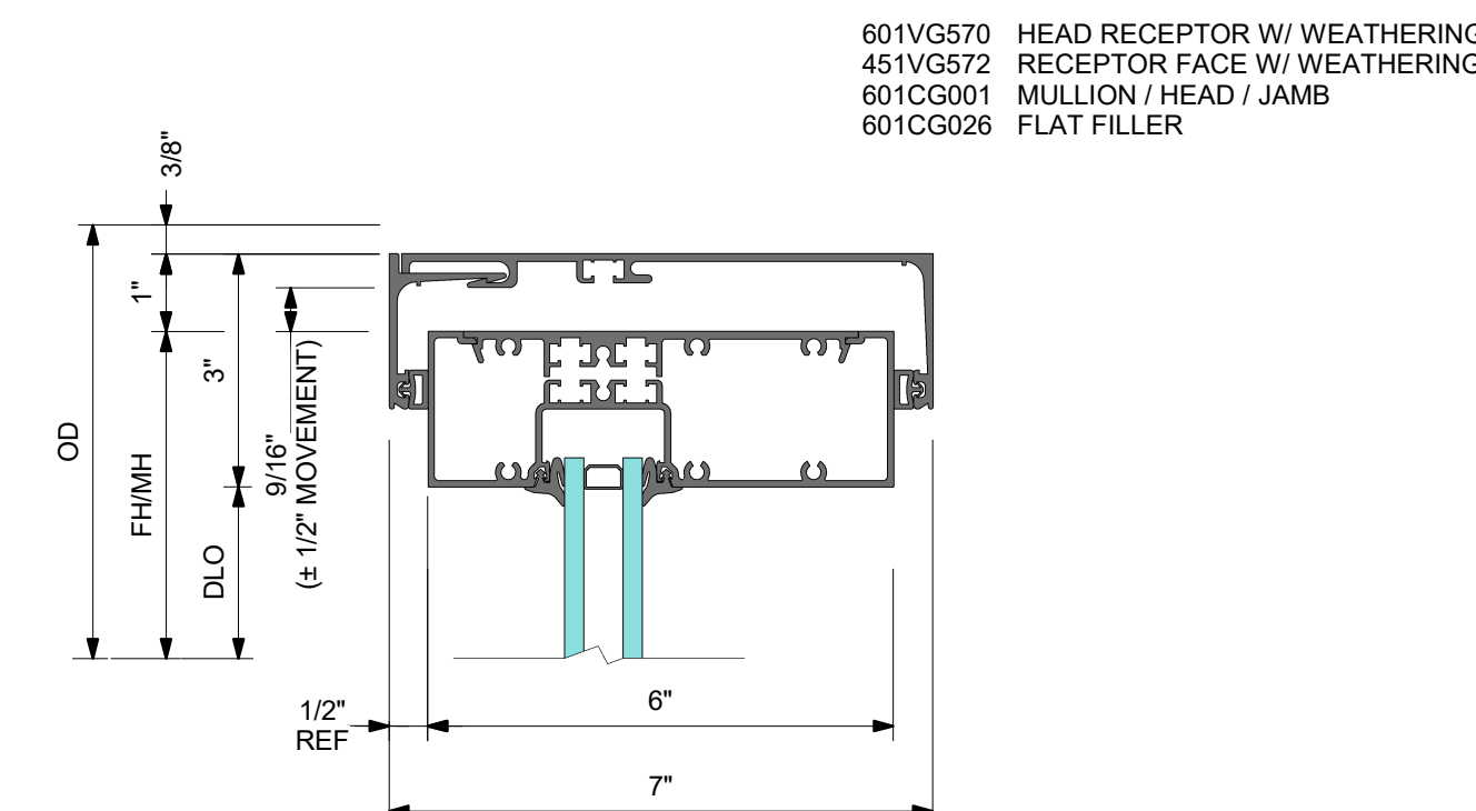
1 DETAIL 1 HEAD WITH RECEPTOR
