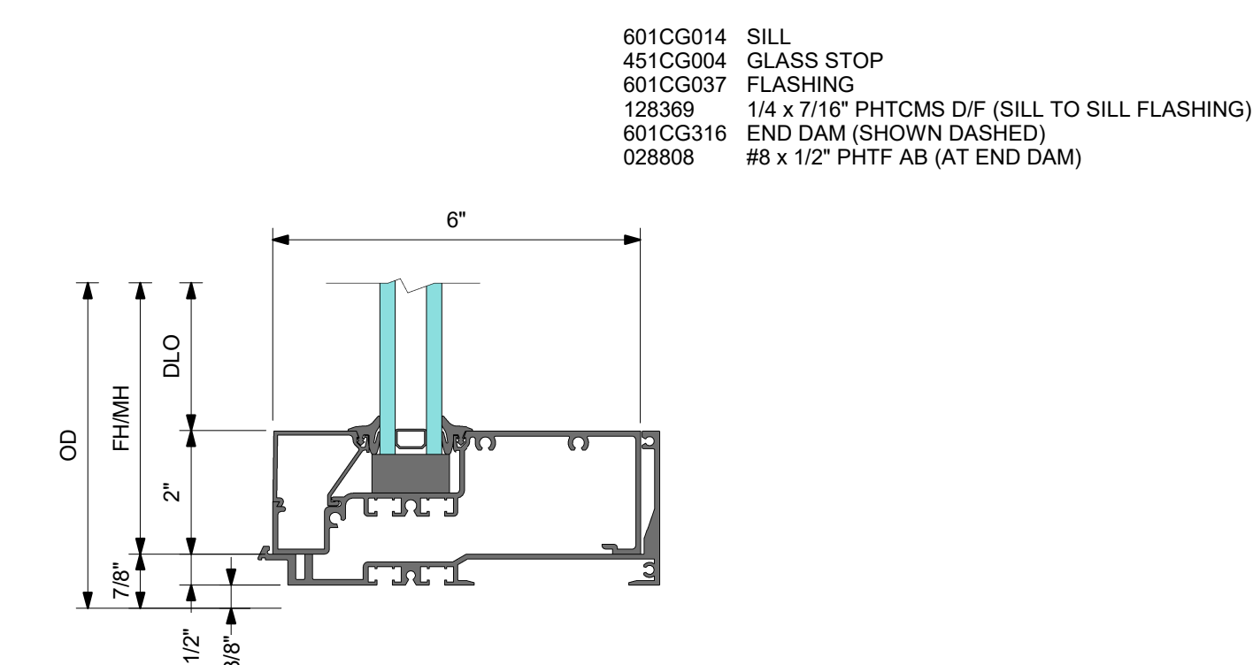
3 DETAIL 3 SILL
