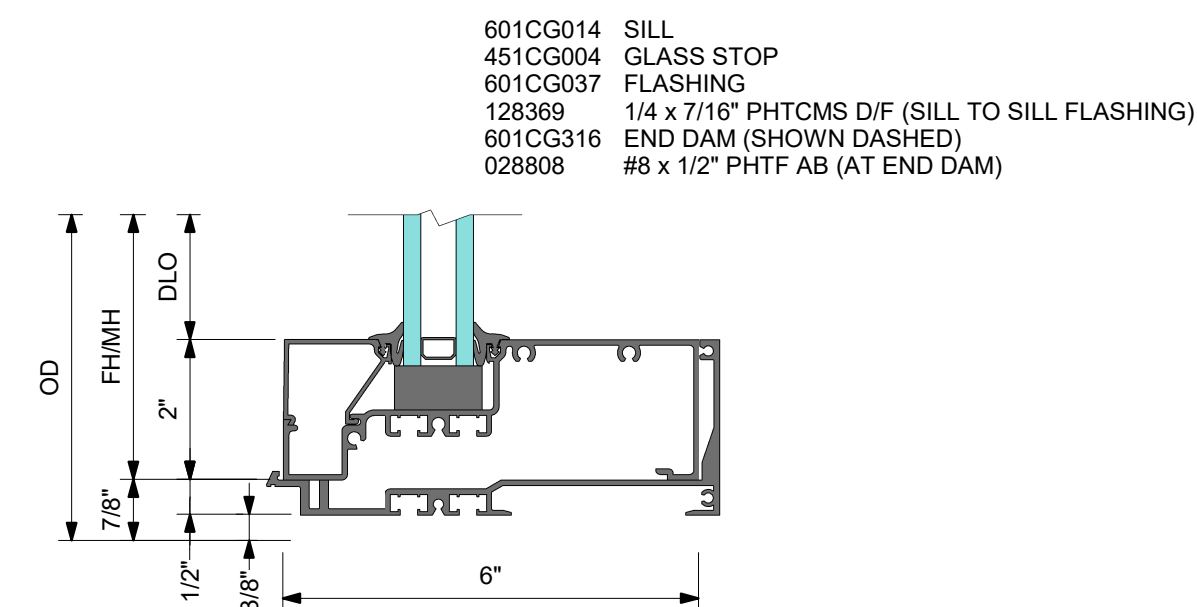
3 DETAIL 3 SILL
