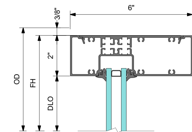
1 DETAIL 1 TRANSOM HEAD
