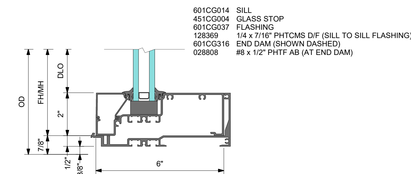
3 DETAIL 3 SILL
