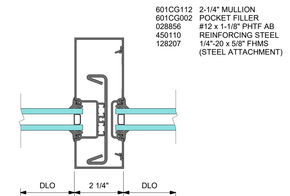
5 DETAIL 5 - 2-1/4" VERTICAL MULLION WITH STEEL
