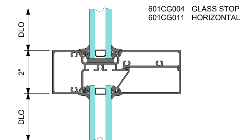
2 DETAIL 2 HORIZONTAL
