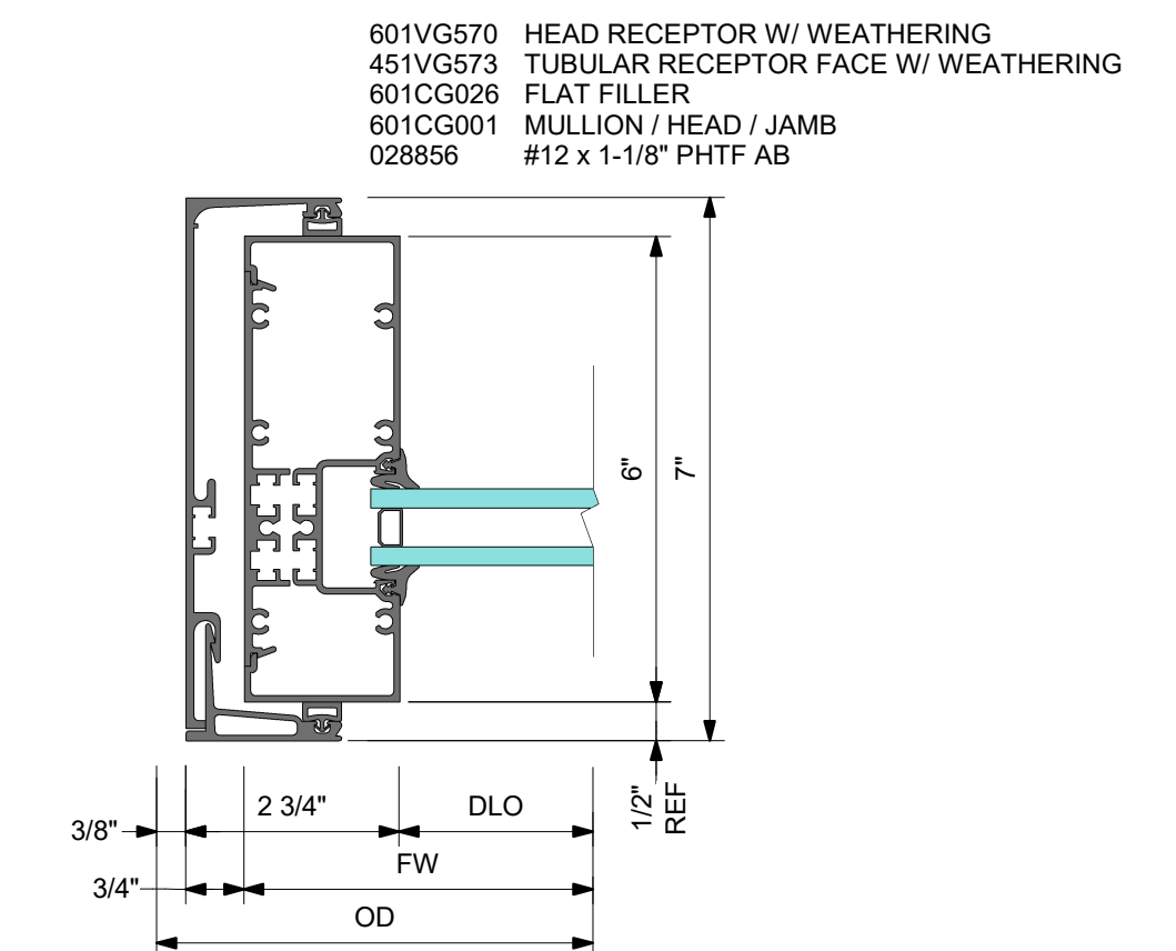
4 DETAIL 4 JAMB WITH HD RECEPTOR
