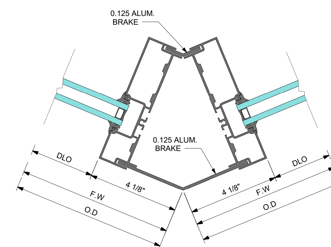
135° OUTSIDE CORNER WITH BRAKE METAL
