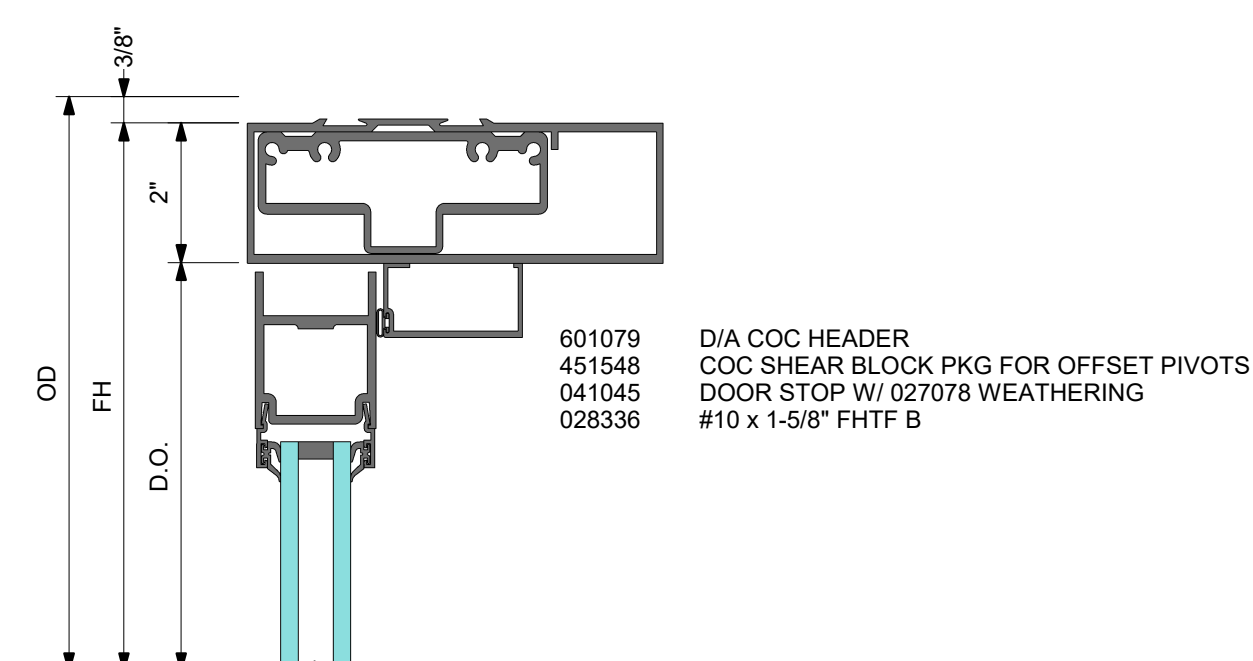
DOOR HEADER WITH KAWNEER CONCEALED CLOSER AND OFFSET PIVOTS
