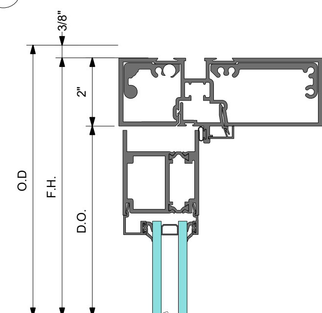
2A DETAIL 2A DOOR HEADER WITH SURFACE CLOSER
