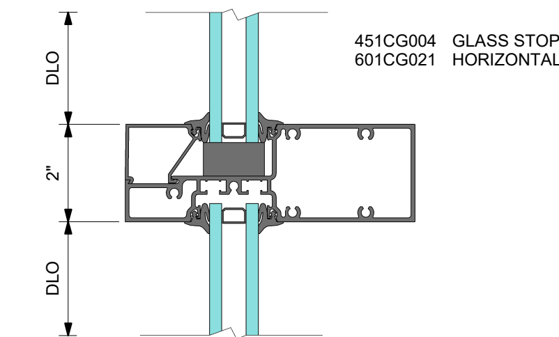
2 DETAIL 2 HORIZONTAL
