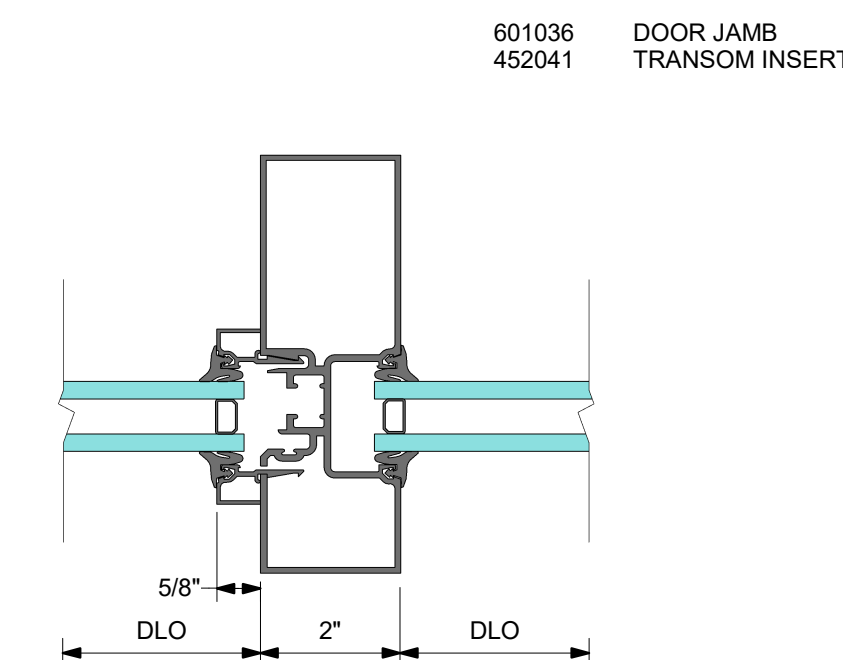
5A DETAIL 5A TRANSOM JAMB WITH SIDELITE
