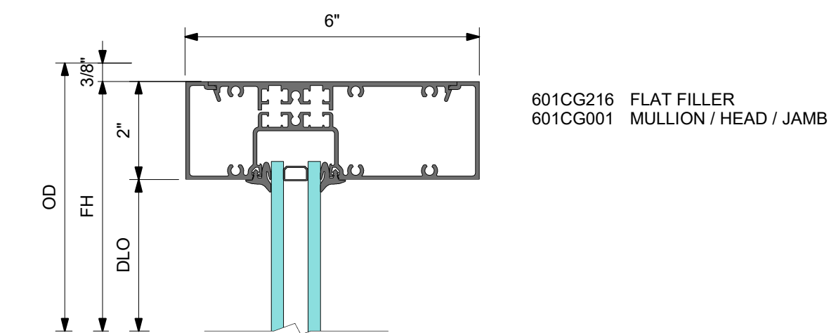
1 DETAIL 1 TRANSOM HEAD
