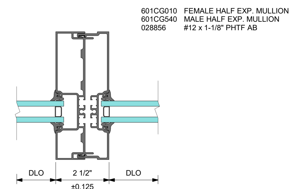
6 DETAIL 6 EXPANSION MULLION
