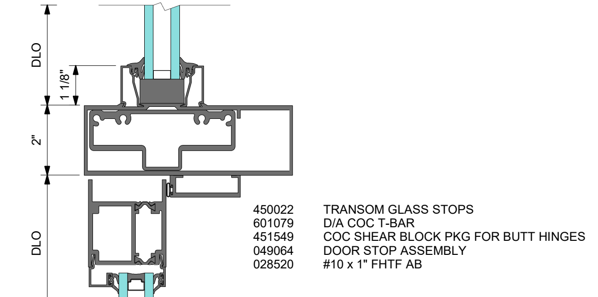
DOOR TRANSOM BAR WITH LCN CONCEALED CLOSER AND BUTT HINGES
