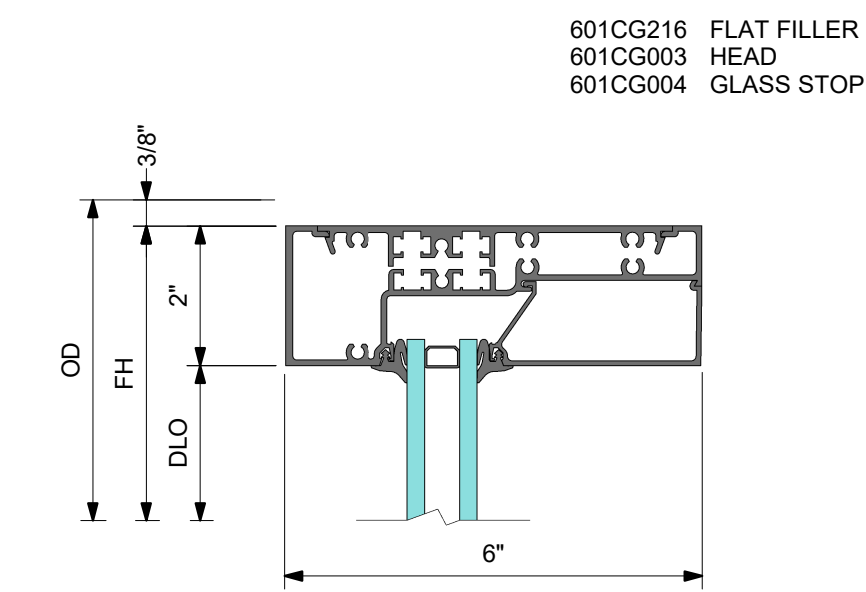
1 DETAIL 1 HEAD
