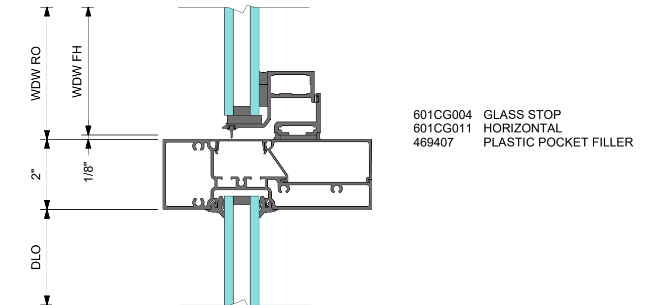
2 VENT SILL
