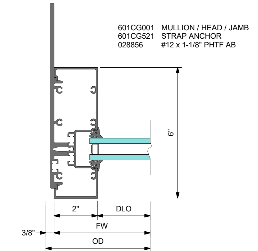
4 DETAIL 4 JAMB WITH STRAP ANCHOR
