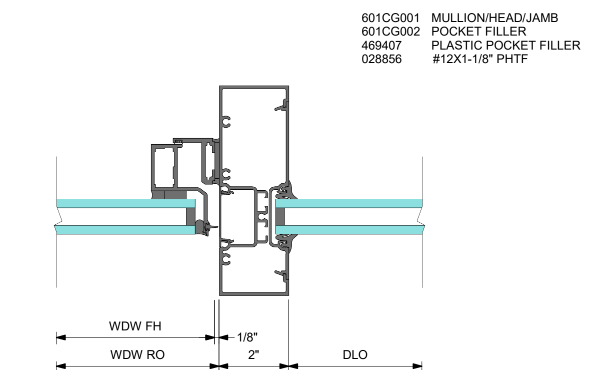
4 VENT @ LEFT
