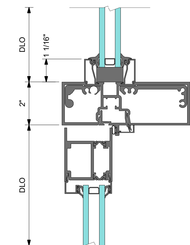
2 DETAIL 2 TRANSOM BAR WITH SURFACE CLOSER
